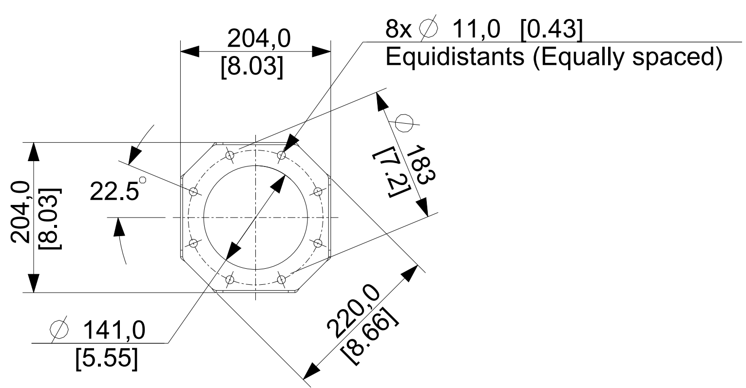
DETAIL : CONTRE-BRIDE / COUNTER FLANGE
