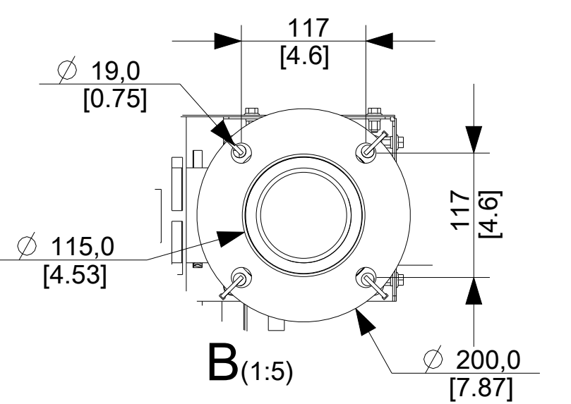
SORTIE ECHAPPEMENT / EXHAUST OUTLET (Detail contre-bride / counter-flange detail)
